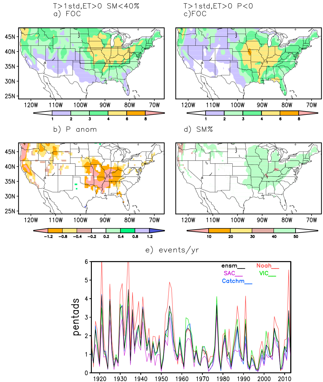
Figure 1. (a) Ensemble mean frequency of occurrence (FOC) of pentads under heat wave flash droughts. Heat wave flash drought is defined as T_{\text{air}} > 1 standard deviation (SD), ET anomaly > 0 , and SM% < 40 . Contours are given by the color bar. The unit is in percent. (b) Composite of P anomalies for pentads under heat wave flash drought defined in Figure 1a. Contours are given by the color bar. Unit is in \text{mm d}^{-1} . (c) Same as Figure 1a but heat wave flash drought is defined as T_{\text{air}} > 1 SD, ET anomaly > 0 , and P anomaly < 0 . (d) Composite of SM% for pentads under heat wave flash drought defined in Figure 1c. Unit is in percent. (e) Number of pentads under heat wave flash drought per year averaged over the box (36–42°N, 80–100°W) for ensemble mean and each model.
